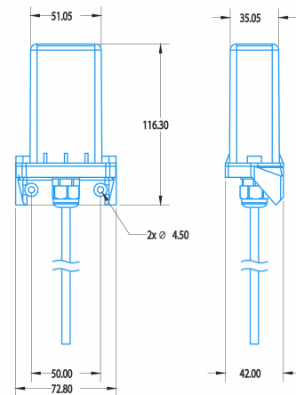
DIMENSION DRAWING OF WIRELESS NODE (Unit: mm)
